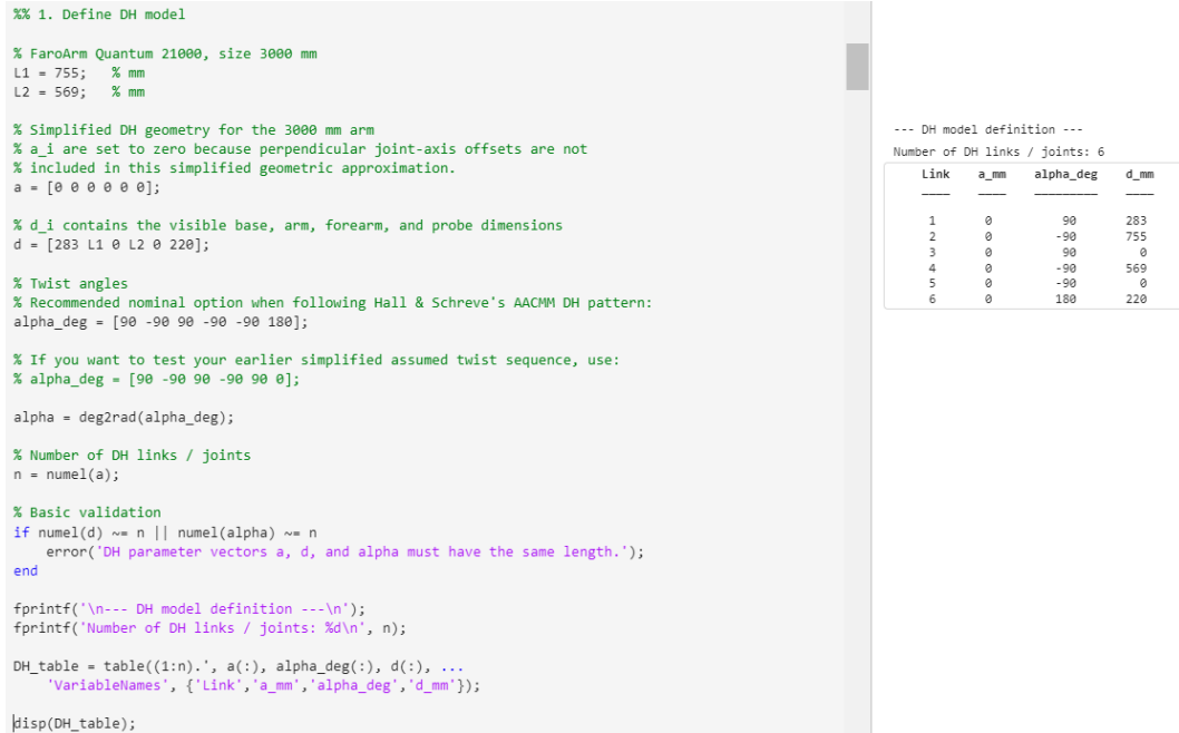
Figure A.1: Error-Propagation Variable Input
